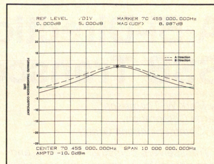
Figure 6. Forward transmission coefficient versus frequency.
