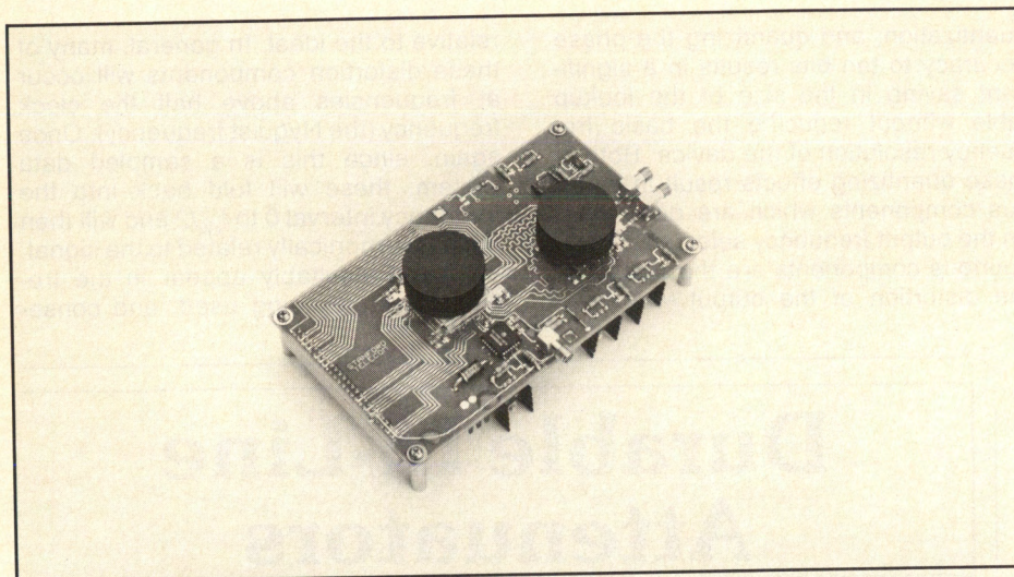
Figure 4. The STEL-2273 DDS board, showing the STEL-2173 NCO chip and the TQ6112 DAC.
