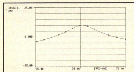
Figure 4. Theoretical forward transmission coefficient (S21).
