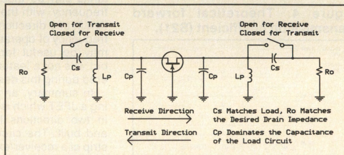
Figure 2. Simplified circuit diagram.
