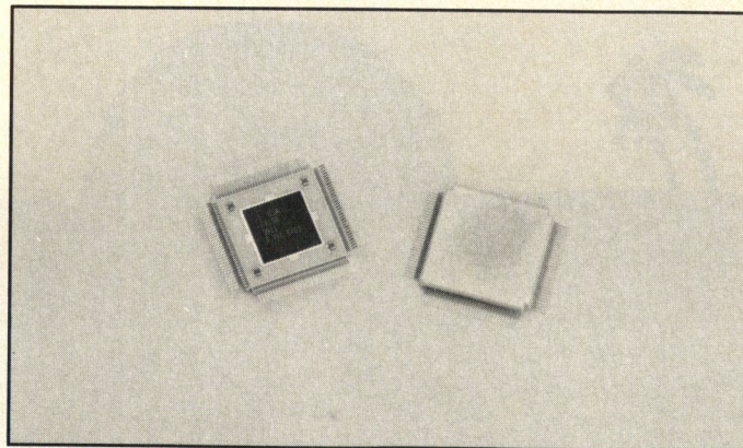
Figure 2. The STEL-2173 is packaged in a 132-pin flatpack. The package is designed with 50 ohm I/O lines for optimum speed, with one ground pin for every two signal pins.
