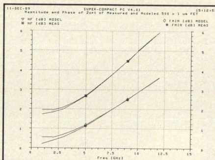
Figure 10. Fit between measured and modeled minimum noise figure and 50 ohm noise figure for a 500 x 1 micron FET after optimization.
