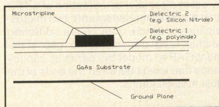
Figure 1. Typical MMIC microstripline structure.
