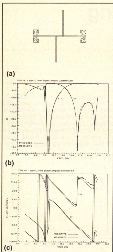
Figure 4. (a) "Simple" GaAs filter structure; predicted versus actual response for (b) S11 and S21 magnitude, and (c) S11 and S21 phase.
