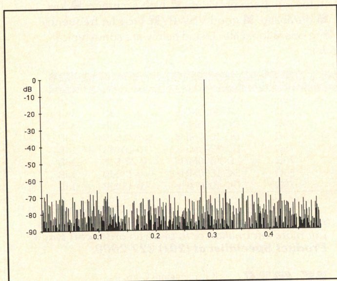
Figure 3. FFT of typical output of STEL-2173, with 10-bit address lookup table.
