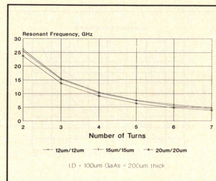
Figure 9. Resonant frequency of spiral inductors as function of track/gap width.
