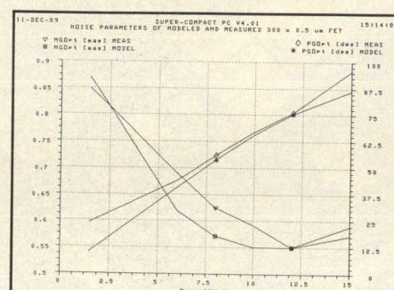
Figure 11. Predicted and measured impedances for minimum noise figure for a 300 x 0.5 micron FET.
