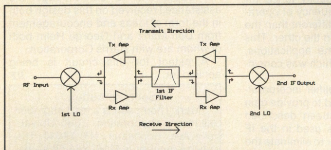
Figure 1. Simplified receiver block diagram showing transmit and receive signal paths.
