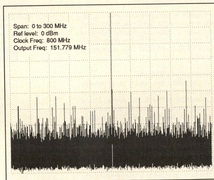
Figure 5. Spectrum plot of typical output of the STEL-2273 board, showing the exceptionally clean output signal for this class of DDS.
