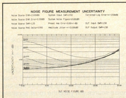
Figure 3. Noise figure measurement uncertainty. DUT input SWR = 1.50, output SWR=1.50 .
