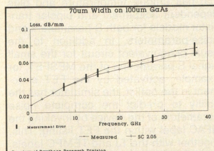
Figure 2. Losses in GaAs microstripline.
