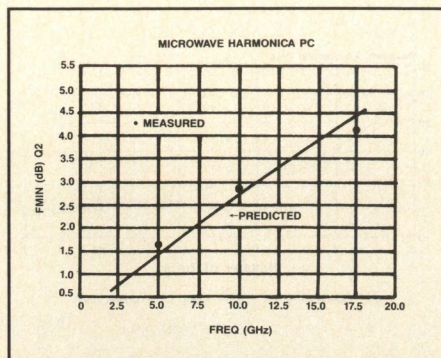
Figure 7. Measured vs. predicted noise figure for a Texas Instruments 0.5 micrometer gate FET.
