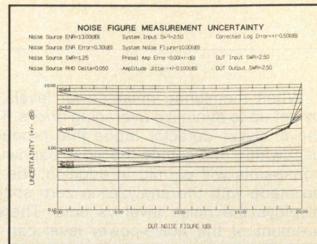
Figure 5. Noise figure measurement uncertainty. DUT input SWR = 2.50, output SWR=2.50 .
