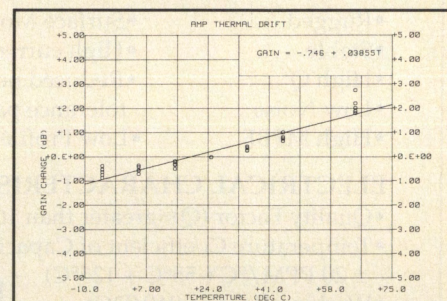
Figure 2. Straight line fit for data.
