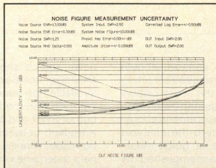
Figure 4. Noise figure measurement uncertainty. DUT input SWR = 2.00, output SWR=2.00.
