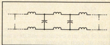
Figure 2. Twisted-wire transmission line equivalent circuit.
