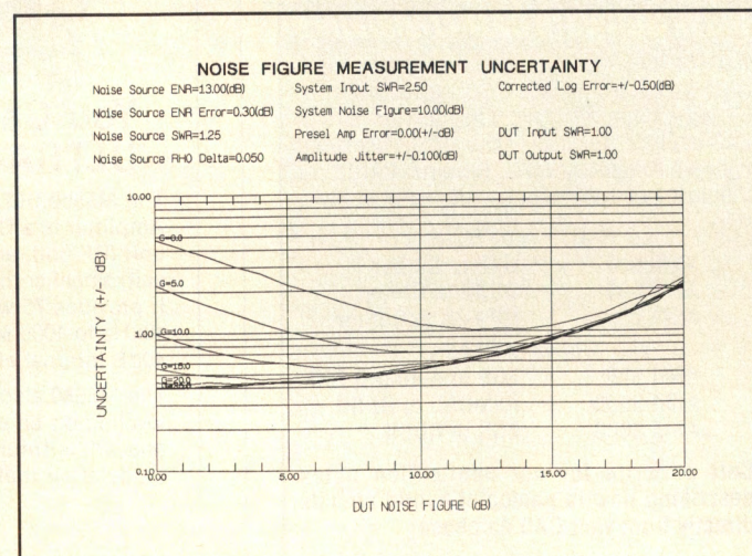
Figure 2. Noise figure measurement uncertainty. DUT input SWR = 1.00, DUT output SWR=1.00 .
