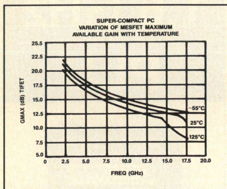
Figure 8. SuperCompact's simulated performance of G_{\max} for the 0.5 micrometer gate FET versus frequency, for three temperatures over the military specified range.
