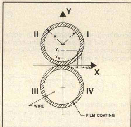
Figure 3. Integration scheme.
