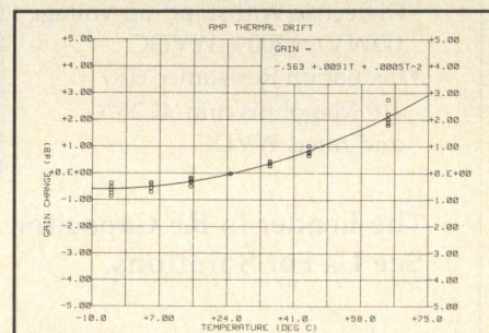
Figure 3. Second order curve fit for data.
