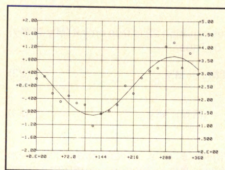
Figure 8. Sine wave fit to noisy data.
