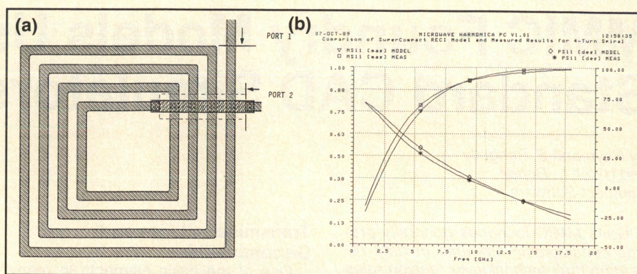
Figure 5. (a) 4-turn spiral inductor typical in MMICs; (b) its simulated and measured S11 magnitude and phase.
