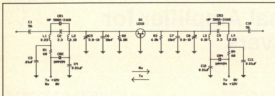
Figure 3. Final schematic.
