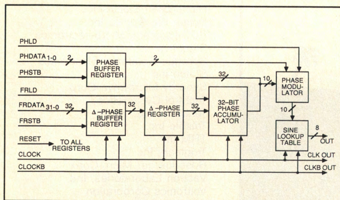
Figure 1. Block diagram of the STEL-2173 GaAs NCO, featuring a 32-bit phase accumulator, BPSK/QPSK phase modulator, and an on-chip sine lookup table.
