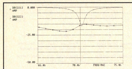
Figure 5. Theoretical input and output return loss.
