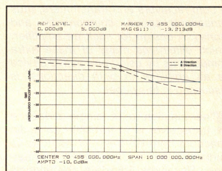
Figure 7. "Input" reflection coefficient versus frequency.
