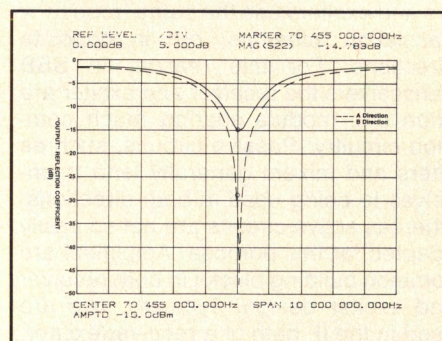
Figure 8. "Output" reflection coefficient versus frequency.
